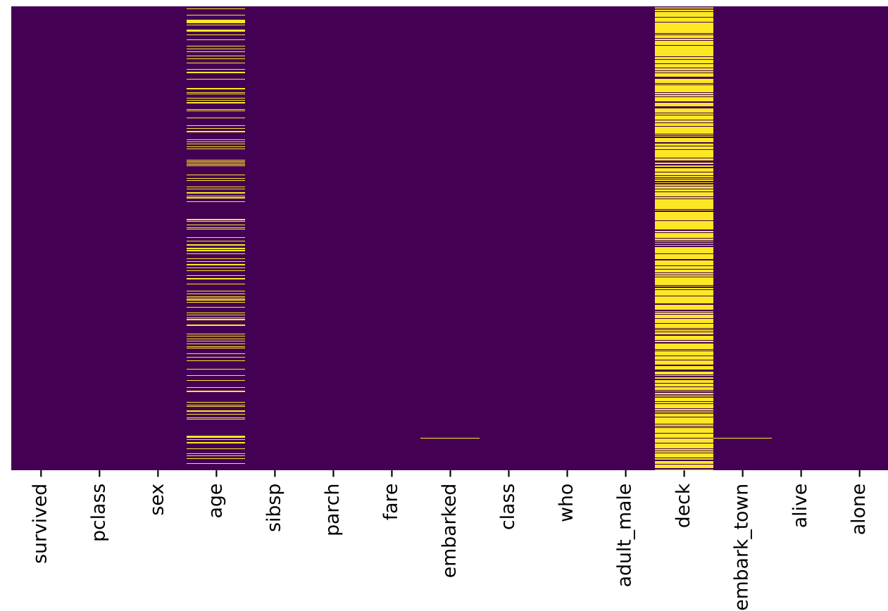
Missing Values Heatmap (Yellow = Missing)
