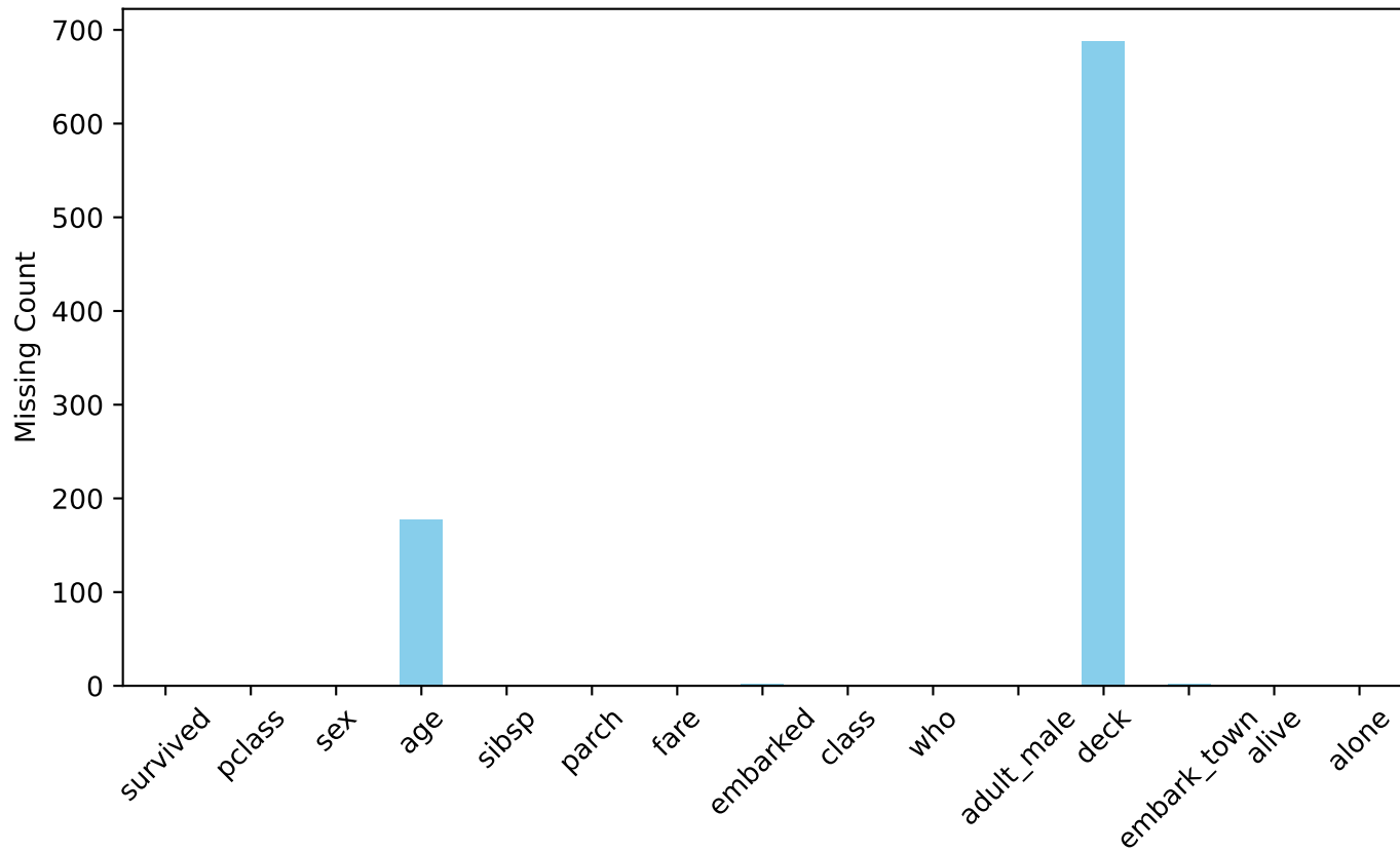
Number of Missing Values per Column
